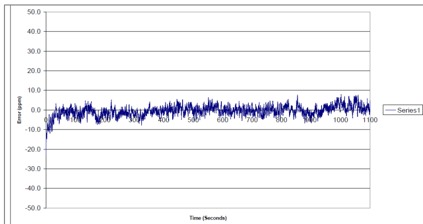
Shunt 1 (Batch 2) Without Heatsink ACV Settling at 19A 430Hz Final Tab Temperature = 44 Deg. C
