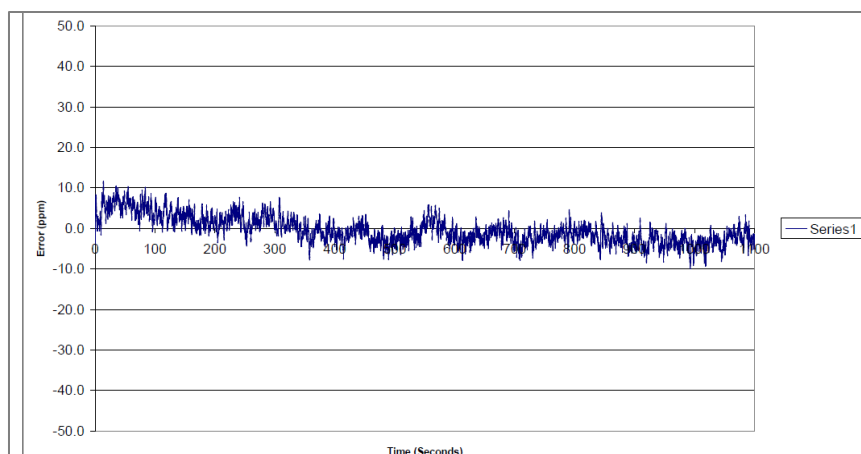
Shunt 12 (Batch 2) Without Heatsink ACV Settling at 19A 430Hz Final Tab Temperature = 45 Deg. C
